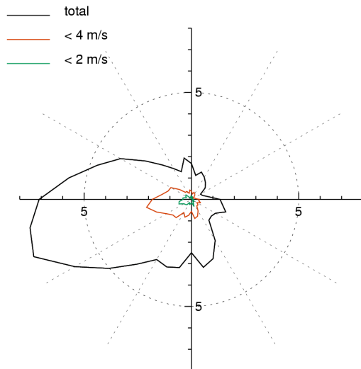
Fig. 7.2.12: Wind rose of Sable Island (west wind system).
