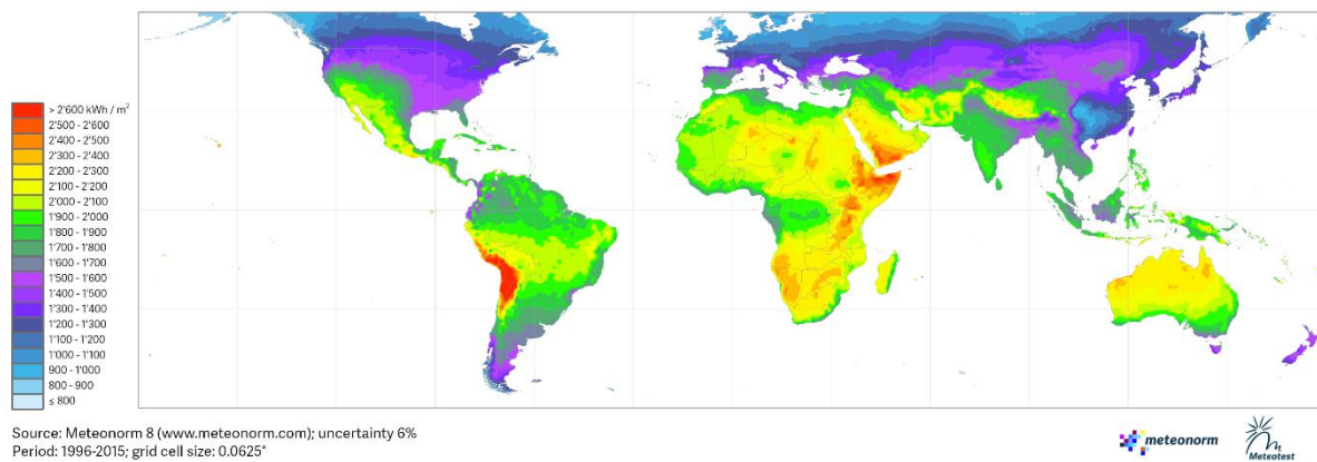
Fig. 3.1.2: Map of yearly sum of global irradiation in kWh/m 2 based on satellite and ground information. Means adapted mainly to the period 1996–2015.
