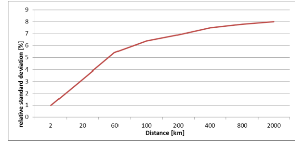
Figure 1: Uncertainty of interpolation of ground measurements vs. distance.
