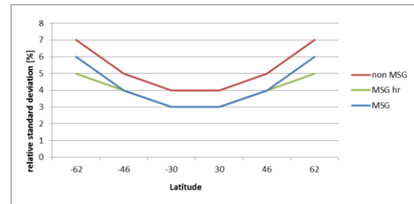
Figure 2: Uncertainty of satellite data in dependence of latitude and source of satellite. MSG= Meteosat Second Generation, hr = high resolution area (Europe).
